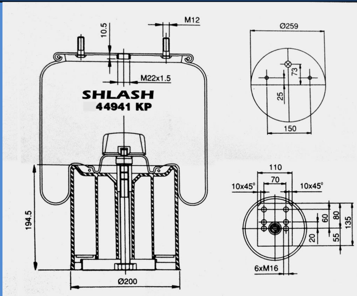
CONTITECH 941 MB WITH METAL PISTON
