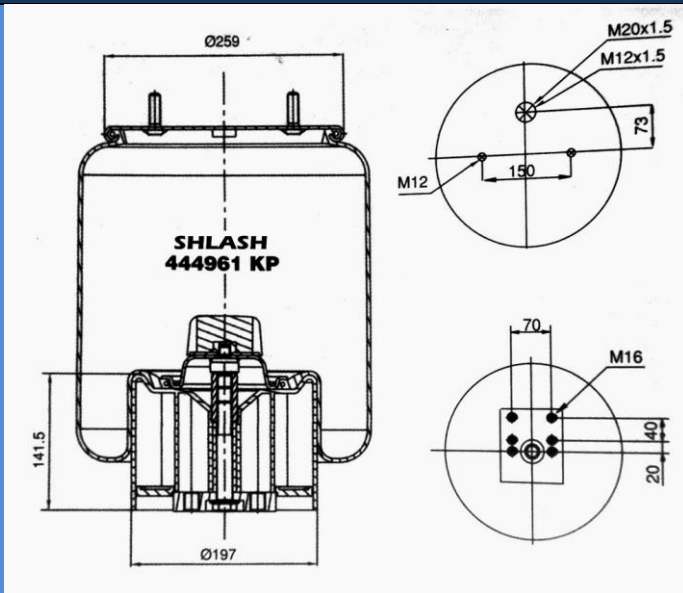
CONTITECH 4961 N P02 (WITH PLASTIC PISTON)
