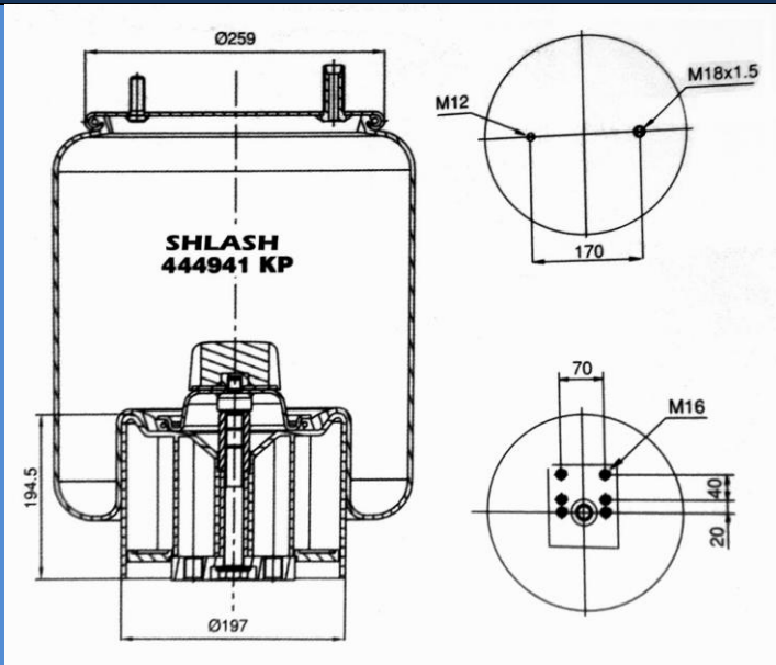
CONTITECH 4941 N P02 (WITH PLASTIC PISTON)
