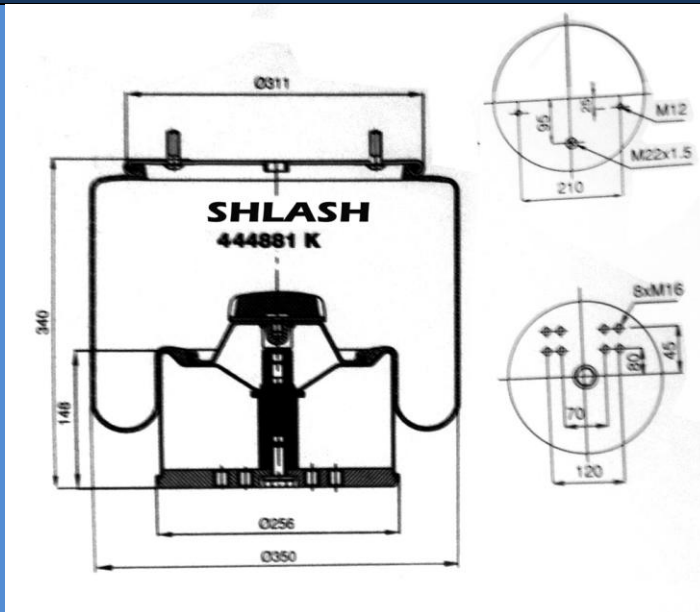
CONTITECH 4881 N P02 (WITH METAL PISTON)
