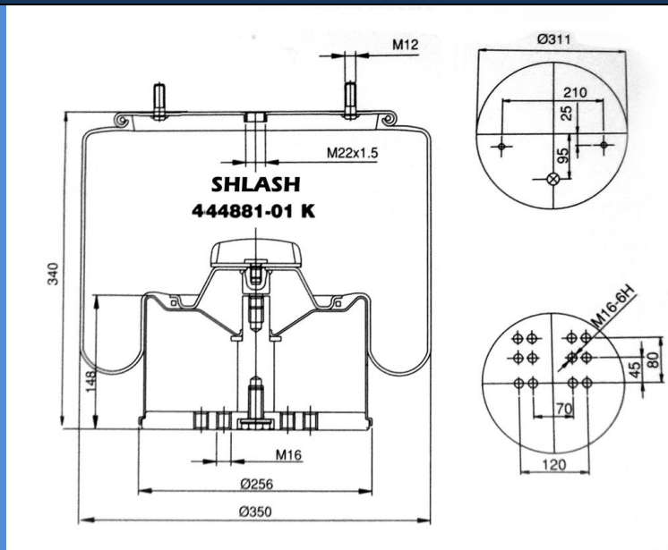
CONTITECH 4881 N P02 (WITH METAL PISTON)
