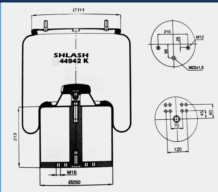
CONTITECH 941 MB WITH METAL PISTON
